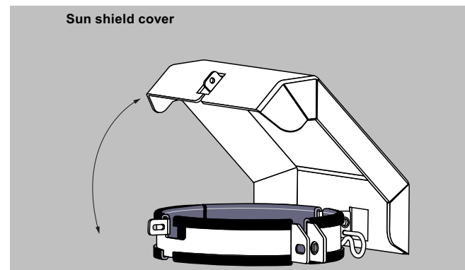
SITRANS LR500 series sunshield
